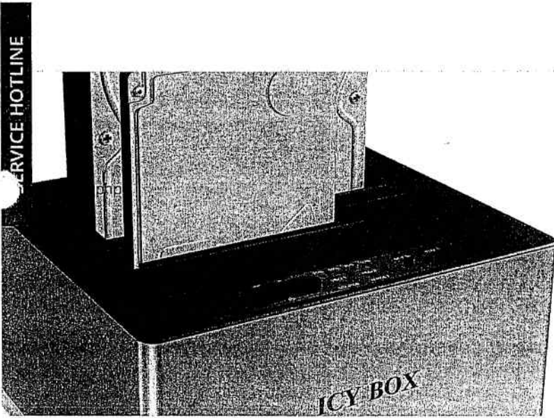
IB-121CL-6G - 2Bay Docking- and Clone Station for 2.5" and 3.5" SATA HDDs with JBOD Function and USB 3.0 with UASP support
